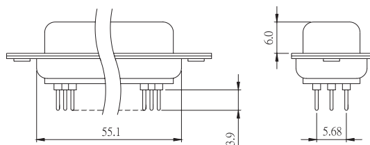
50 POSITION FEMALE
